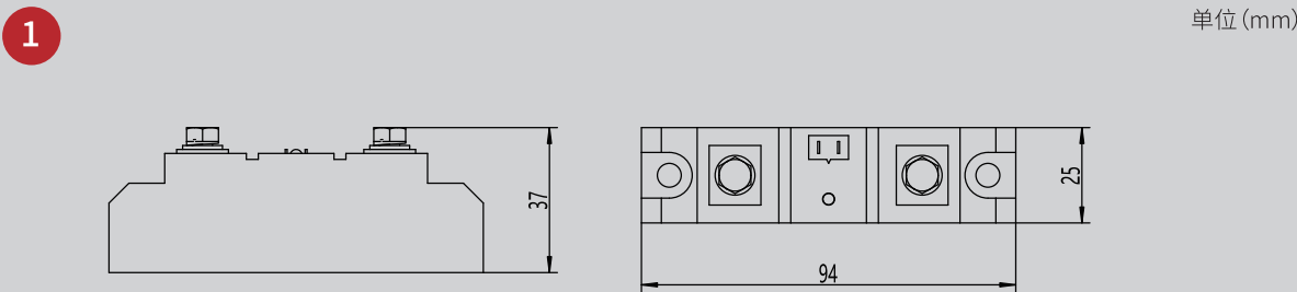
(SAM4040D-120D/SAM6060D-120D尺寸图如图1所示)
